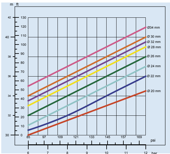
Jet length
