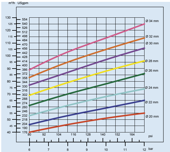
Pressure/Flow
